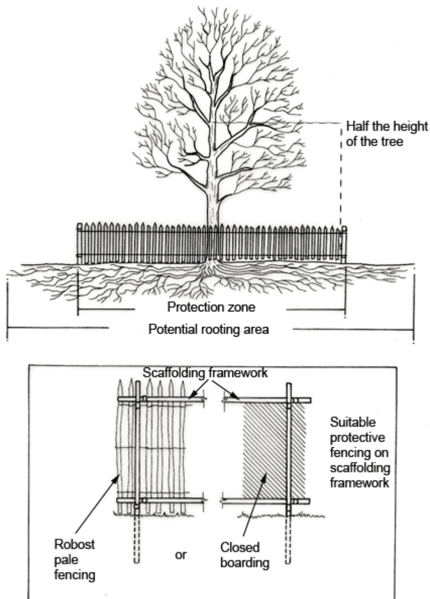
Figure RT4 Avoiding damage to trees
