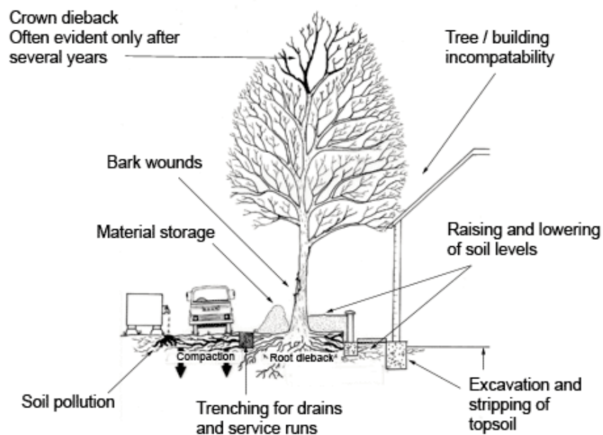
Figure RT3 Damage to trees during construction works
